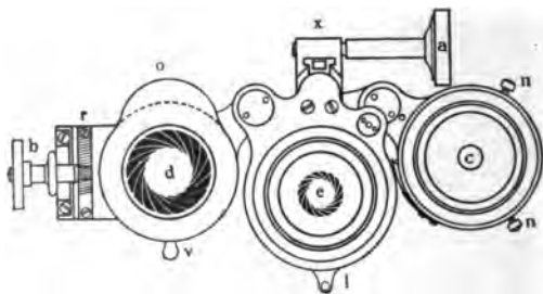
Fig. 51c. Complete Substage. Top view, with condenser and lower iris diaphragm swung out of optical axis.
